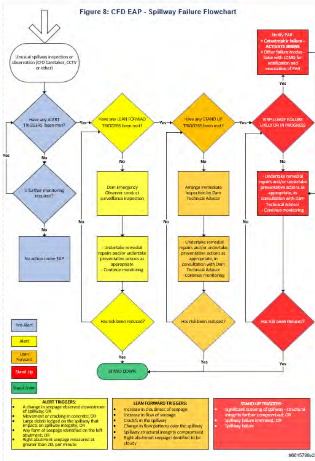
Figure 8: CFD EAP – Spillway Failure Flowchart
