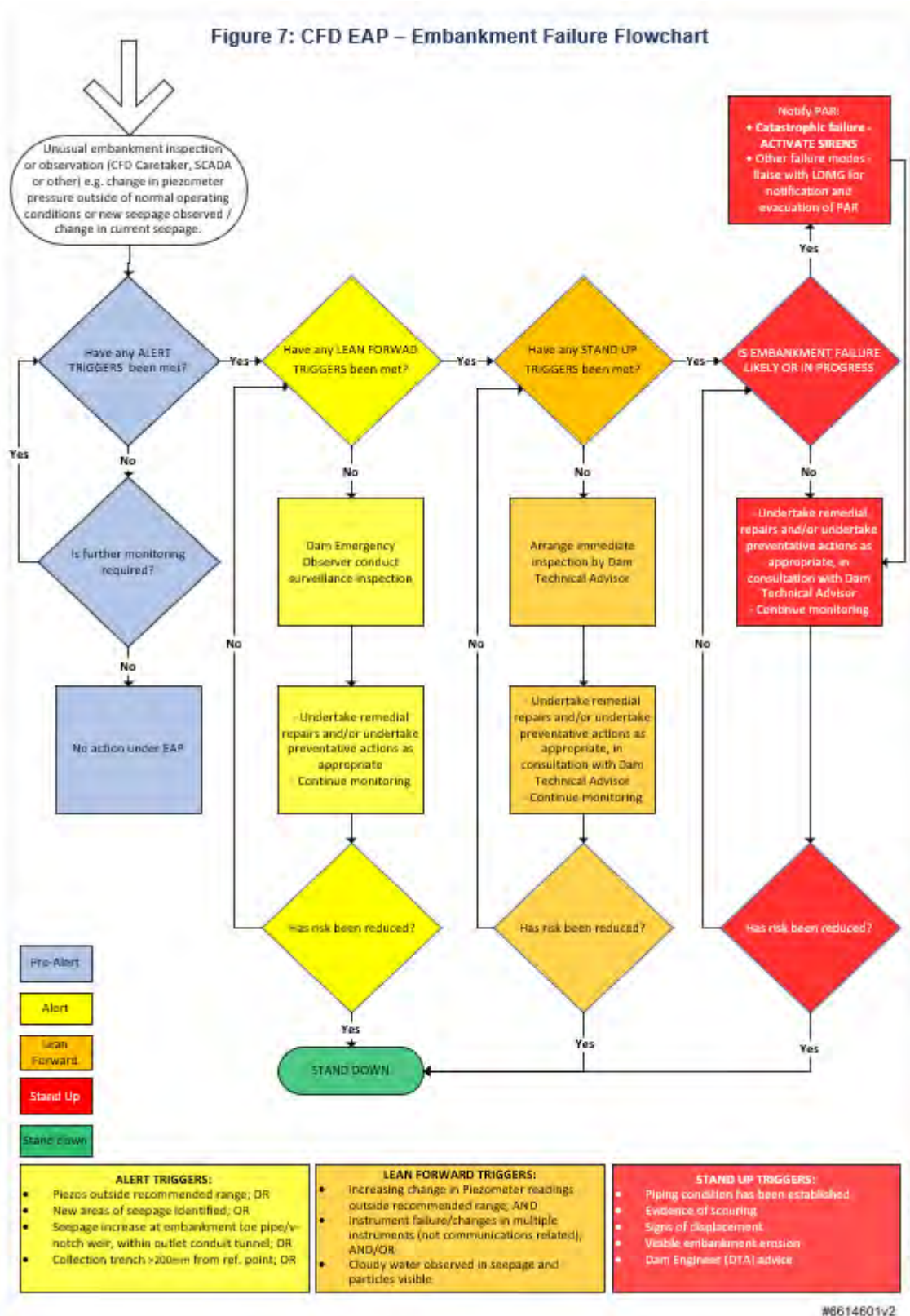
Figure 7: CFD EAP – Embankment Failure Flowchart
