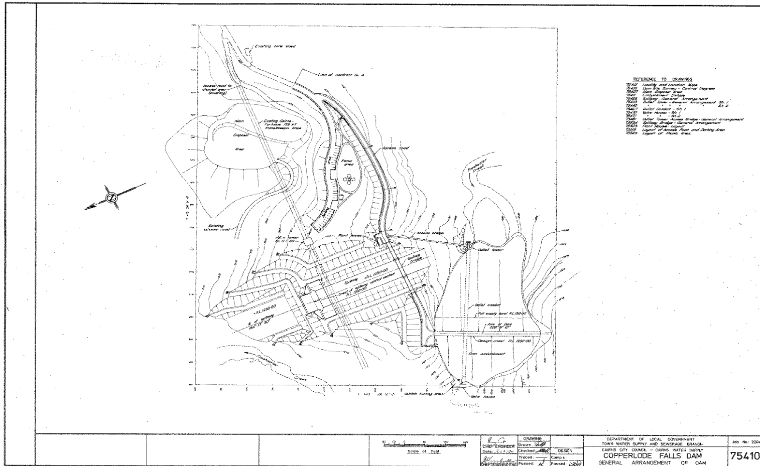
General Arrangement of Dam #3220693
