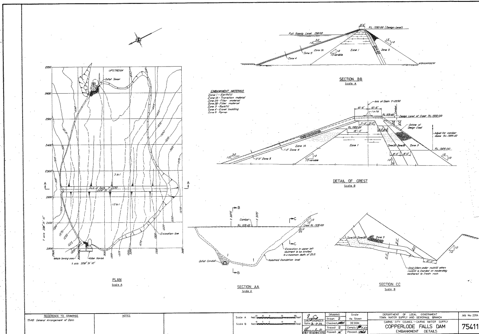
Dam Embankment Details #3220745
