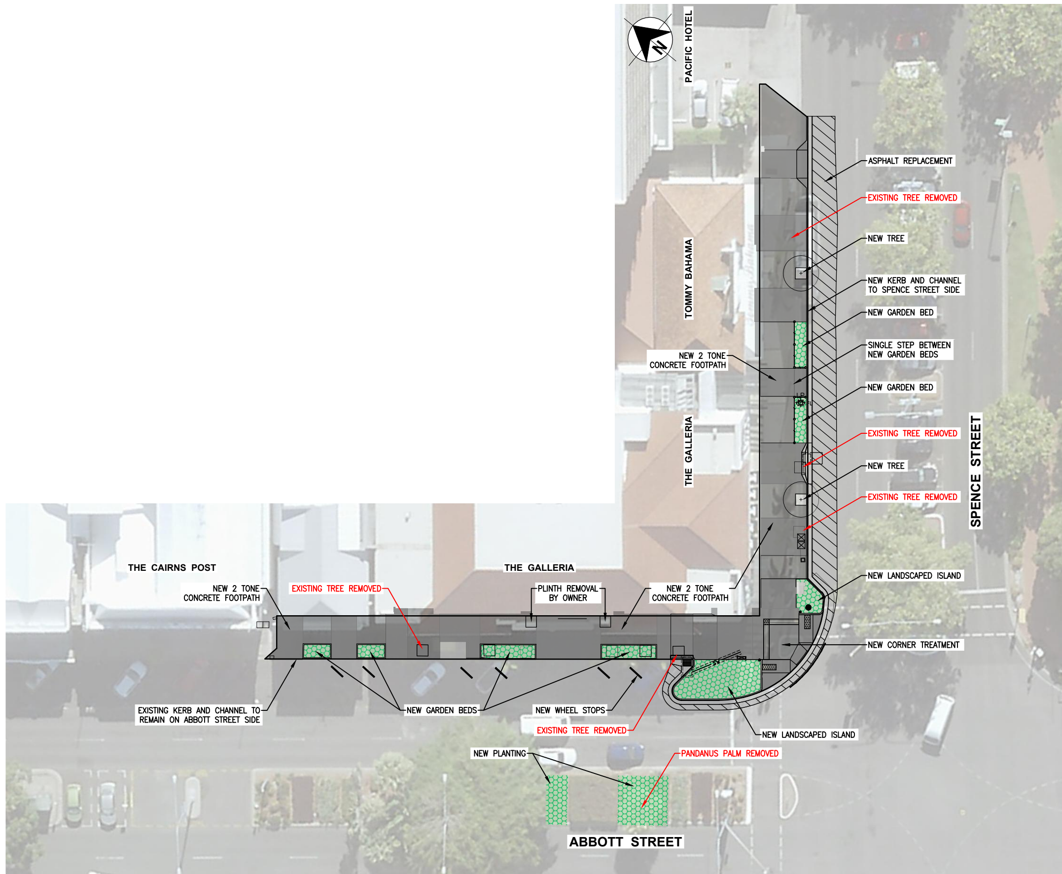
PLAN SCALE 1:200@A1
