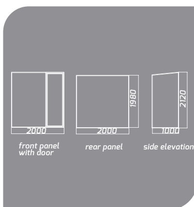
Figure 2. Steel frame for base unit
