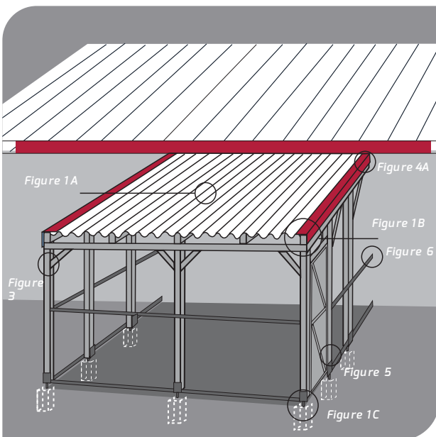
Figure 9. Patio type structure. This shows the basic building structure prior to the addition of solid weatherproof wall cladding on parts of the enclosure (to provide the cat with shelter) and prior to the addition of other features (platforms, climbing planks, scratching posts, beds etc) as described in the text.
