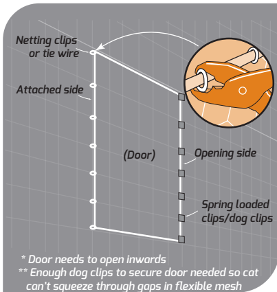
Figure 8. Design and construction of door
