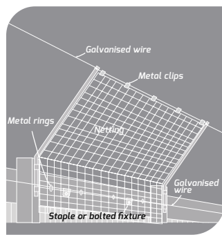
Figure 5. Securing the netting
