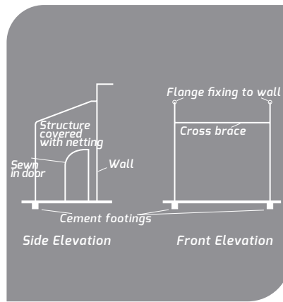
Figure 7. Tubular steel enclosure
