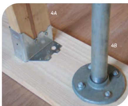
Figure 4A. Fixing method for timber
